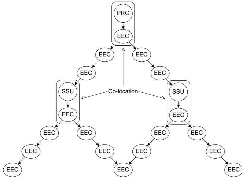
Figure 2: Inter-node distribution architecture
