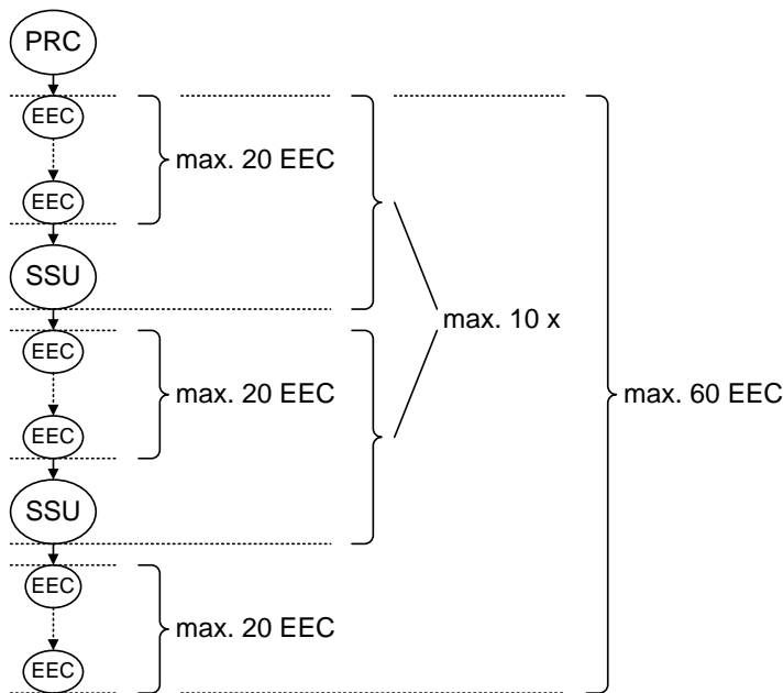
Figure 3: Synchronization reference chain for SyncE and SDH (ITU-T Rec. G.803)
