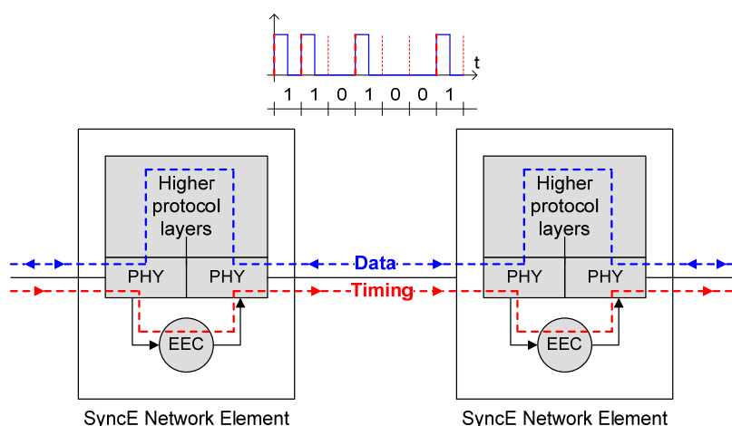
Figure 1: Frequency transfer over the physical layer
