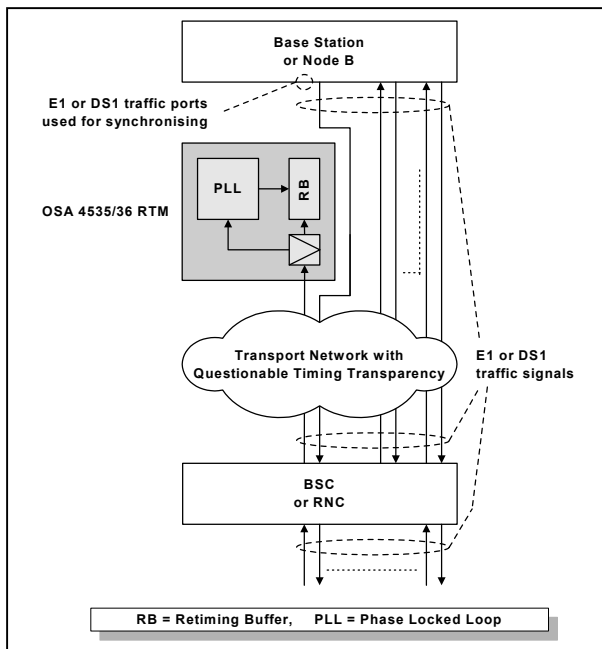
Figure 7: Base station synchronised by regenerated E1 or DS1 signals
