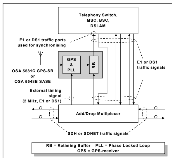
Figure 4: Re-timing used for synchronising a digital switch.
