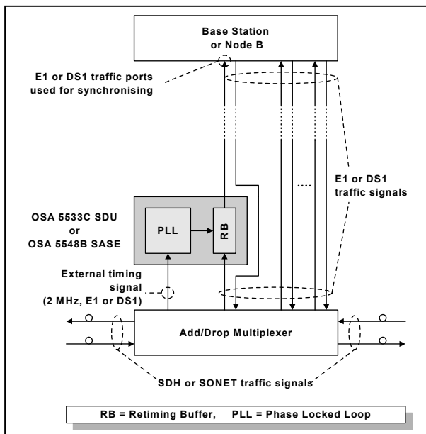
Figure 5: Re-timing used for synchronising a base station.
