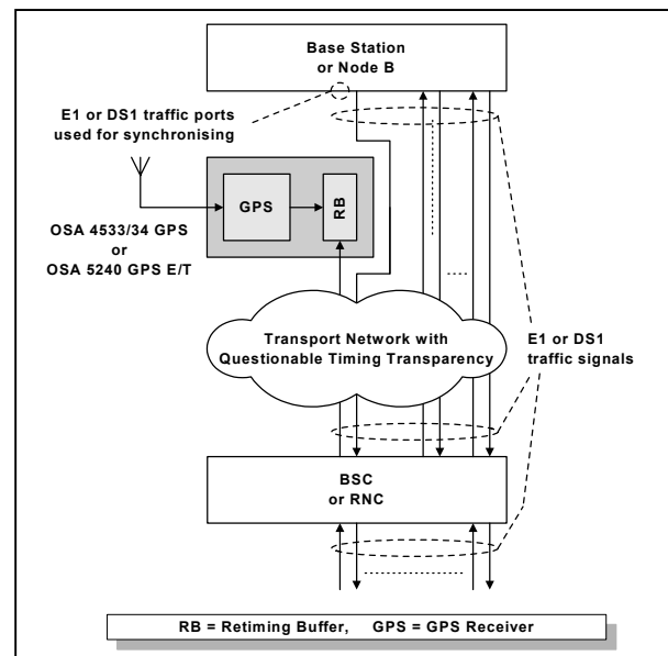
Figure 6: Base station synchronised by the GPS.
