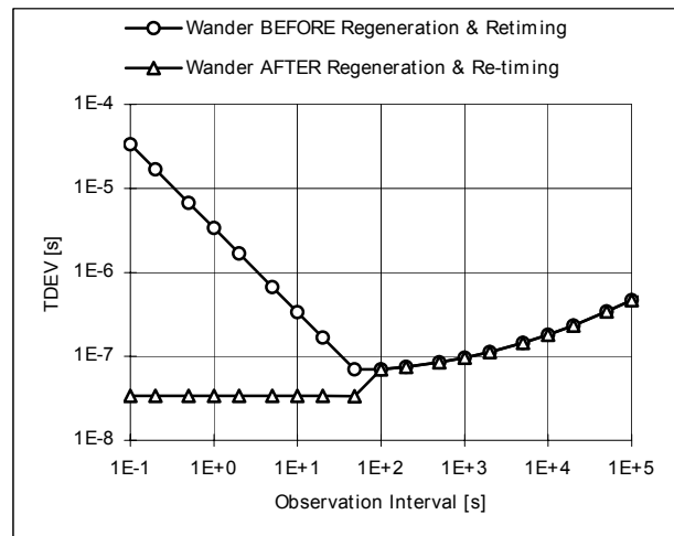
Figure 8: Regenerating capability of a 3 mHz PLL
