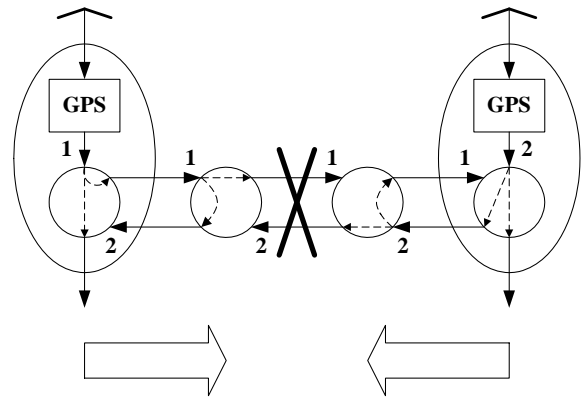
Figure 4: Link failure in an A-type cell.
