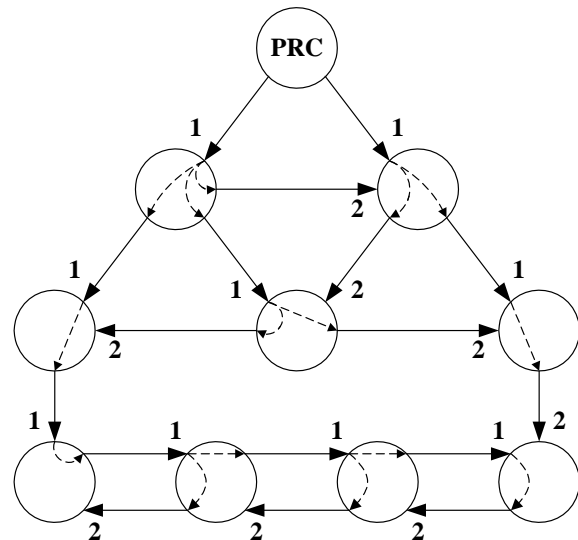
Figure 1: Classical synchronization network.
