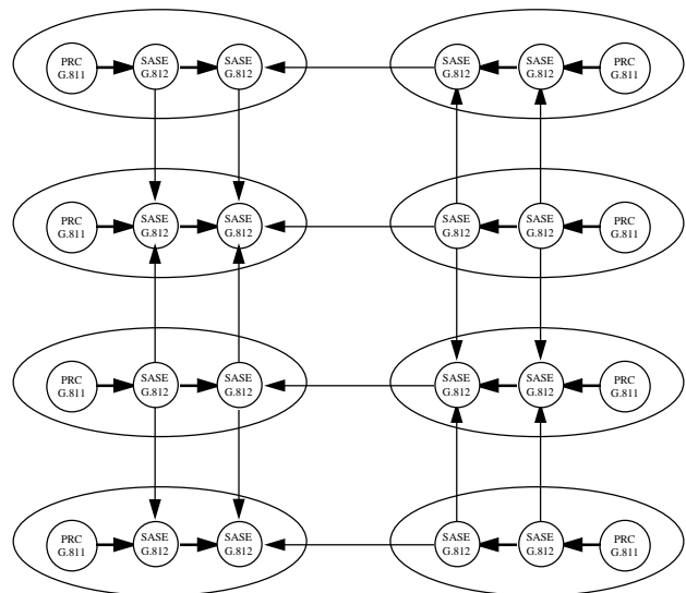
Figure 4 : Distributed synchronisation subnetworks
