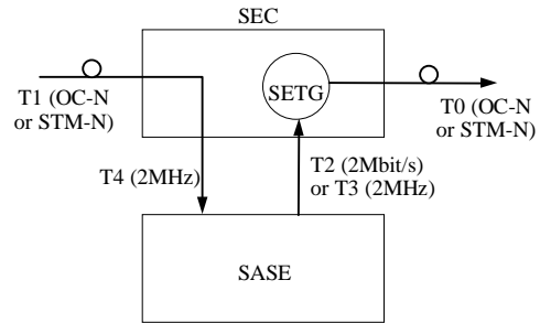
Figure 6 : Intermediary SASE in a large ring or a long chain of NEs
