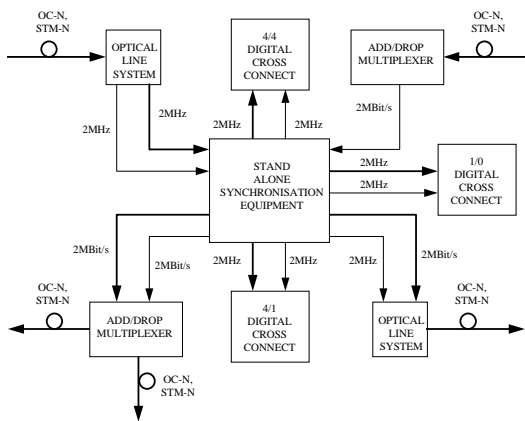
Figure 6 : Network element intra-node synchronisation
