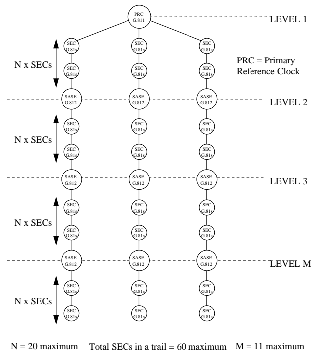
Figure 1: Synchronisation network reference trails
