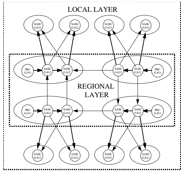
Figure 3 : Distributed synchronisation network architecture
