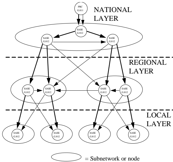
Figure 2 : Centralised synchronisation network architecture
